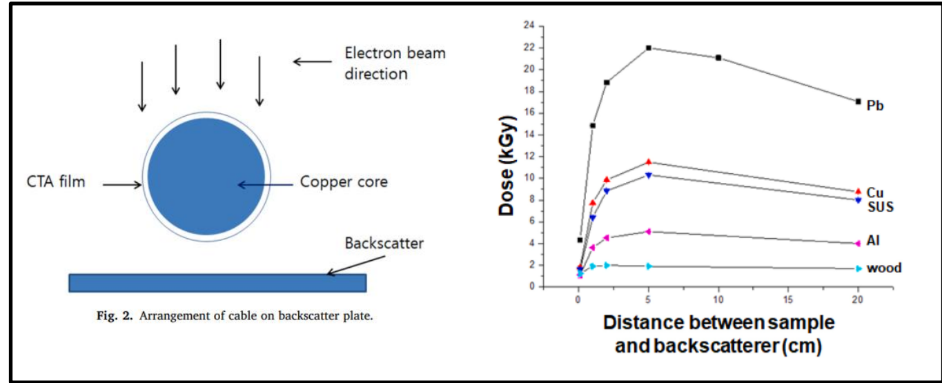
Relation of backscattering and distance between sample and back scatter: Plate Size: 80 × 80 cm 2 (Seung-Tae Jung, 2022)
