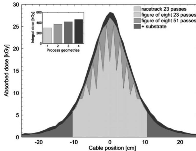
Distributions of mean doses per pass of the cable in Fig. 6 irradiated with four geometrical setup.
